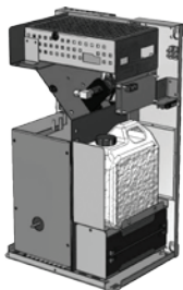
Internal isometric
